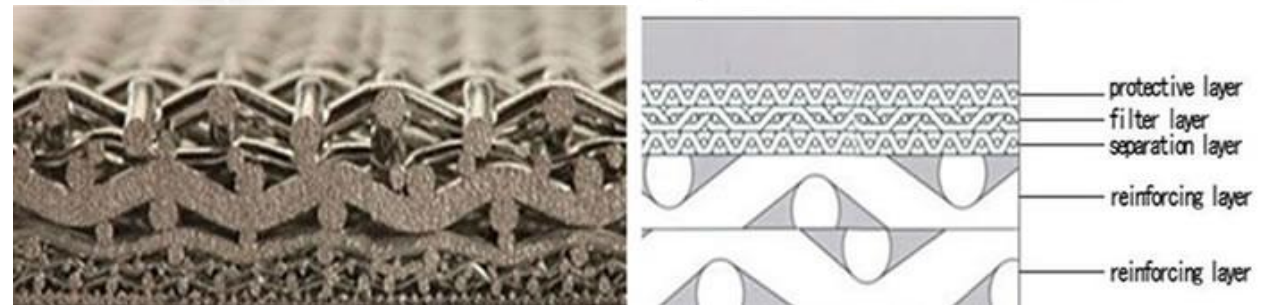
5-layer sintered wire mesh
